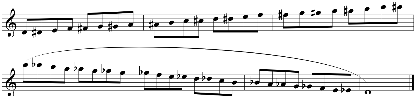
Chromatic Scale
